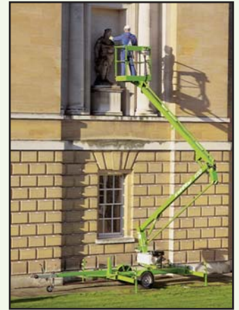
The TM34's manual outriggers are both cost effective and simple to set up.
