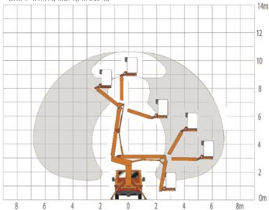
Load of working cage up to 200 kg
